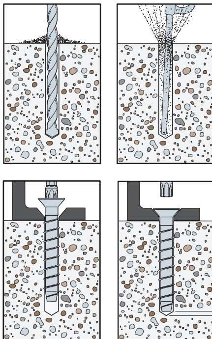
Minimum overdrill. See table.
